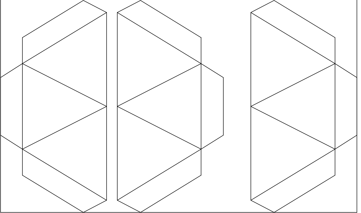
Partial hexagon panel sections without window outlines
